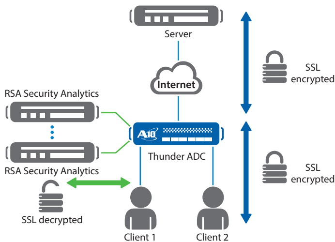
Figure 1: Thunder ADC decrypts and forwards traffic to RSA Security Analytics.
